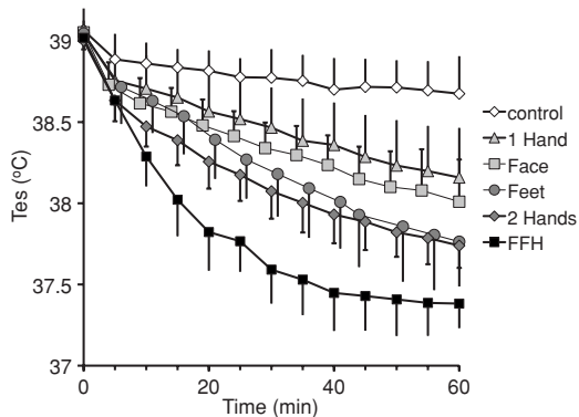
Fig. 4 T_{es} versus time during recovery after exercise in thermally stressful conditions; the effect of cooling the various combinations of glabrous skin regions ( n=8 , mean \pm SD). FFH: foot, face, and hand cooling.
