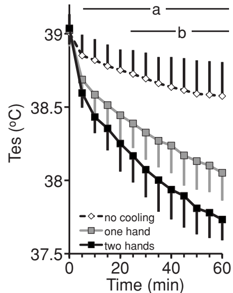
Fig. 2 T_{es} versus time during recovery after exercise in thermally stressful conditions. Treatments: control (no cooling), heat extraction from one hand, and heat extraction from two hands ( n=17 ). Heat extraction entailed the combined application of a heat sink to the glabrous skin of the hand and subatmospheric pressure to the entire hand (mean \pm SD). t -test results: (a) control versus one hand, p<0.001 ; (b) one hand versus two hands, p<0.005 .
