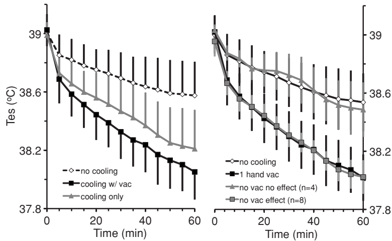
Fig. 3 T_{es} versus time during recovery after exercise in thermally stressful conditions; the effect of cooling one hand, with or without application of subatmospheric pressure. Left: group results n=12 . Right: cooling only (no pressure differential) group data sorted according to effect and compared with the complete data set for one hand cooling with a pressure differential and no cooling. In eight subjects the response to cooling-alone resembled the response to cooling with subatmospheric pressure. In four subjects, the response to cooling-alone resembled the no treatment response.
